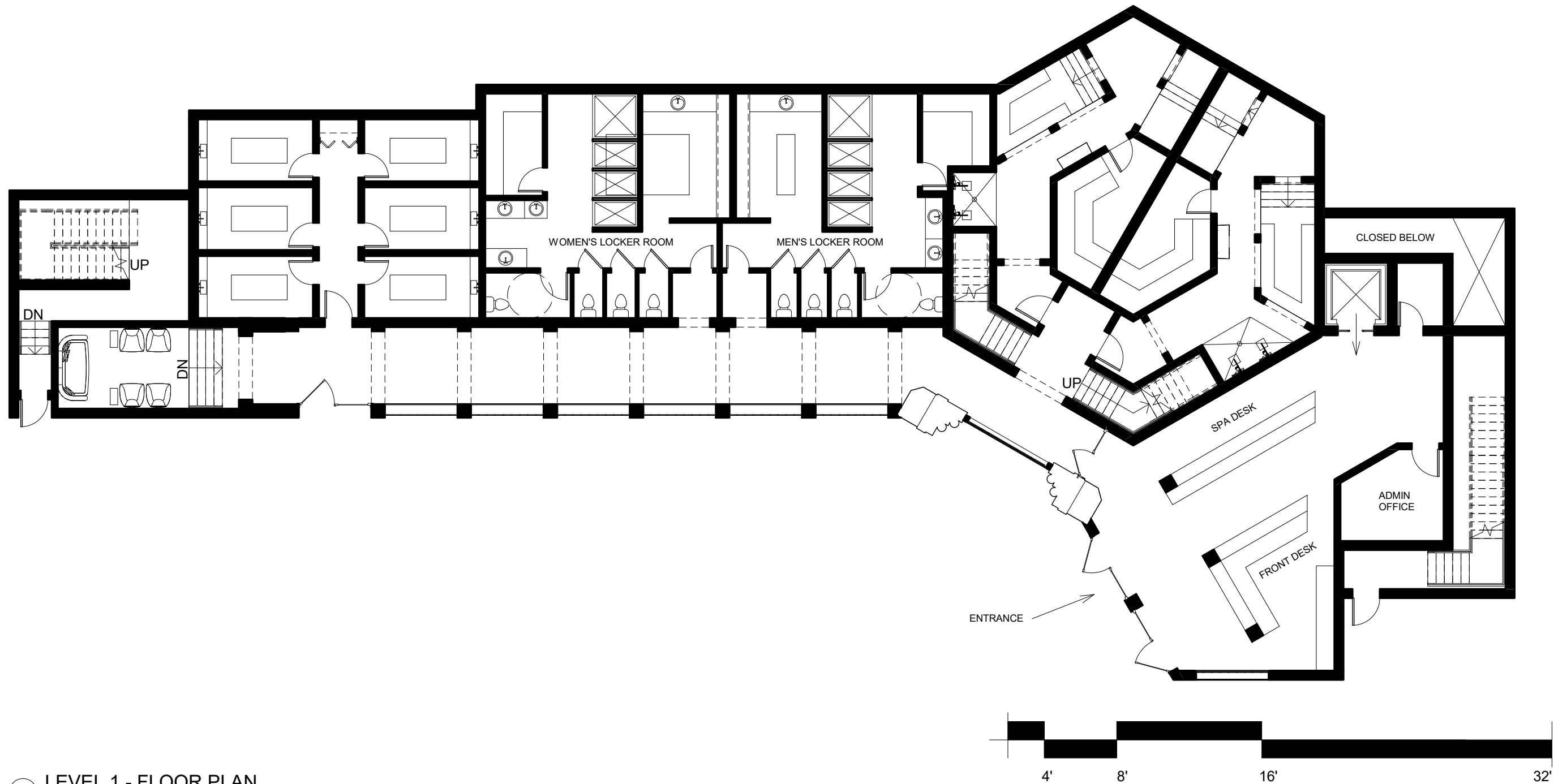
① LEVEL 1 - FLOOR PLAN 1" = 12'-0"
